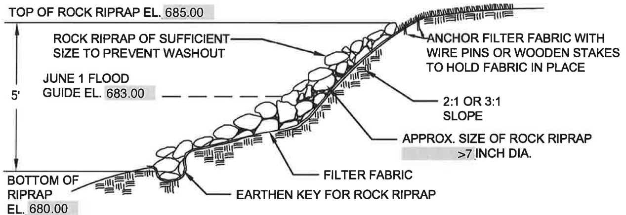
SECTION SHOWING STABILIZED SHORELINE
