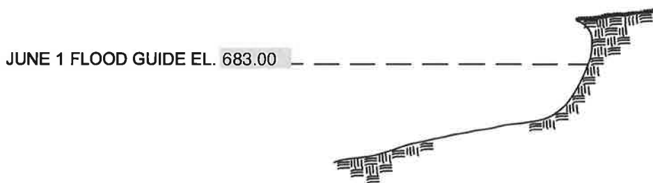
SECTION SHOWING EXISTING SHORELINE
